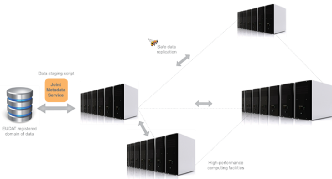
Figure 4: B2STAGE Process
