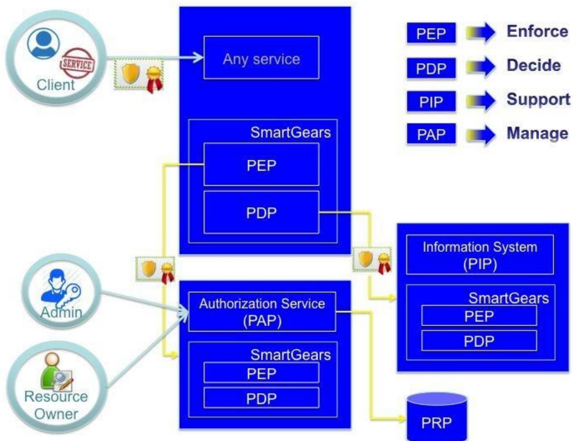
Figure 3.11: Authorization Architecture
