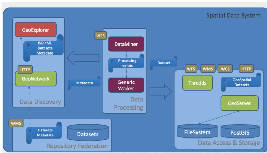
Figure 3.17: Spatial Data Repositories Architecture
