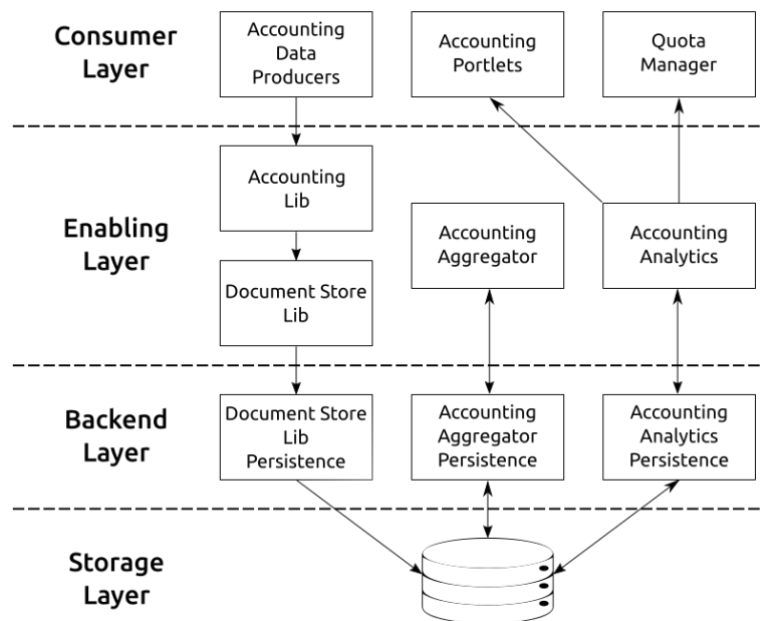
Figure 3.12: Auditing Architecture
