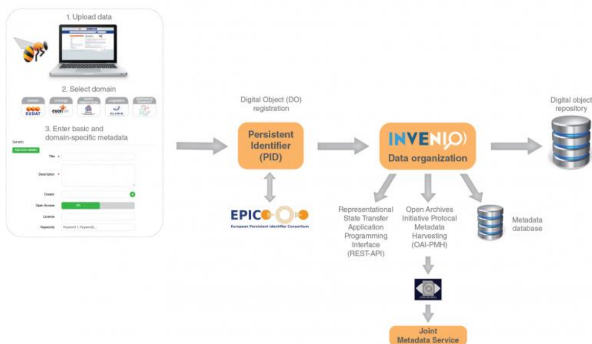
Figure 6: B2SHARE Architecture
