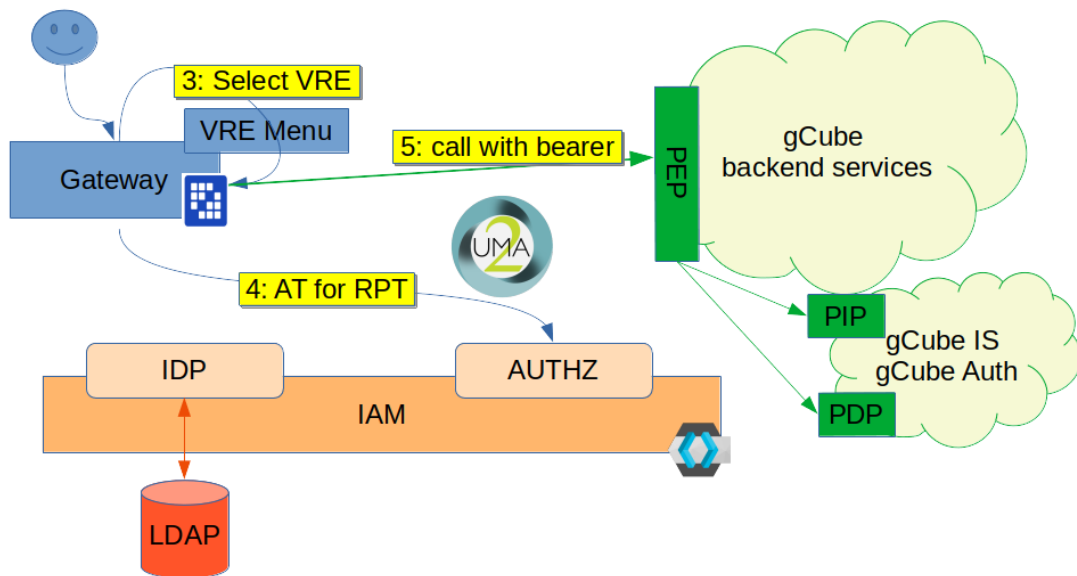
Figure 3.10: Authorization grant to access context (VO or VRE)
